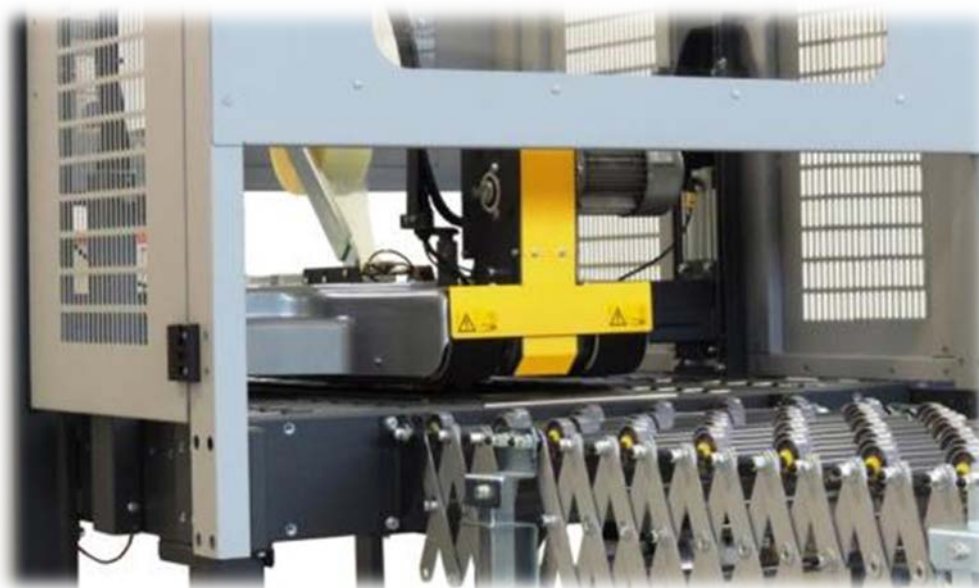
Detail for the minimum position of machine taping head.
